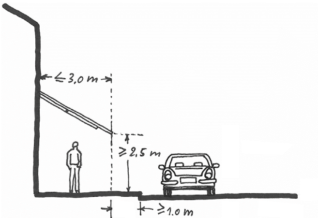
Figure 2 : Saillies mobiles
