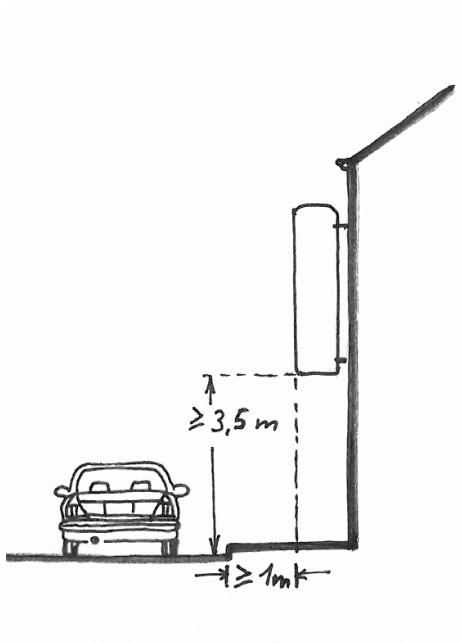
Figure 1 : Installation des supports publicitaires
