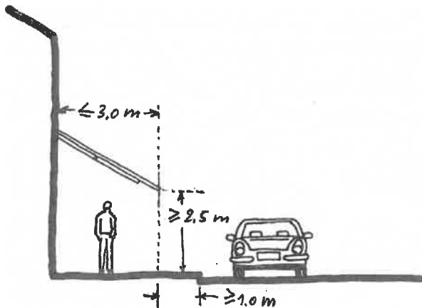
Figure 2 : Saillies mobiles
